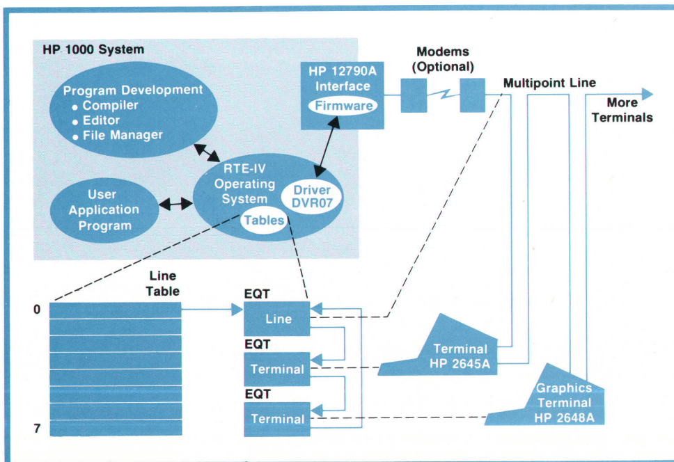
Fig. 1. Multipoint allows many terminals to share one communications line. In HP 1000 multipoint, terminals are assigned conventional RTE equipment table (EQT) and logical unit (LU) numbers, and are treated like other peripherals. The communications line also has EQT and LU status. All of the EQT numbers of a particular line are stored in a linked list that describes that line.
